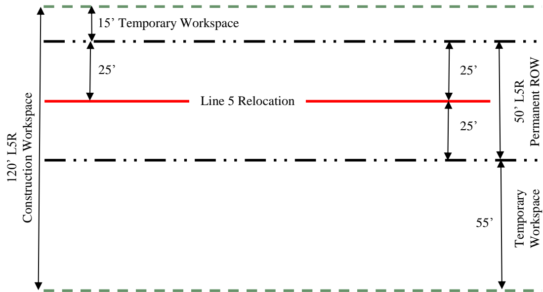
Figure 3.1.1-1: Typical Construction Workspace—Uplands
