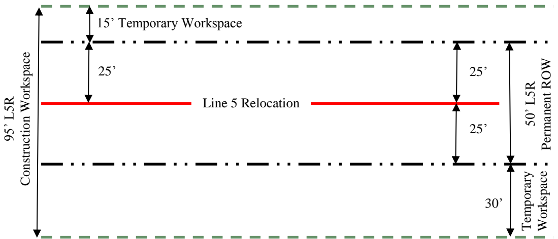
Figure 3.1.1-2: Typical Construction Workspace—Wetlands
